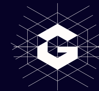
Subtracted G
