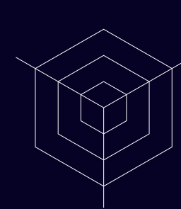
Tesseract
