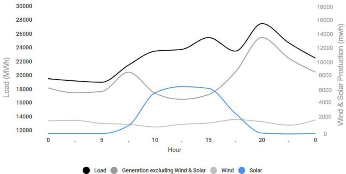
Figure 5: California's electrical load on April 17, 2017 25
