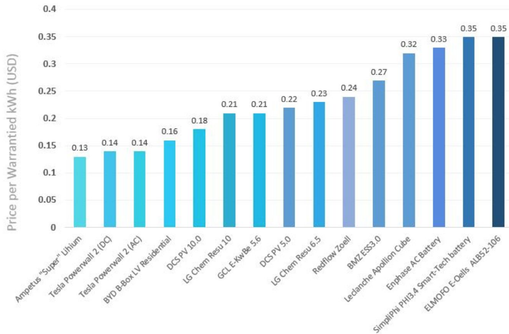
Figure 6: Average Price of Energy Storage 31
