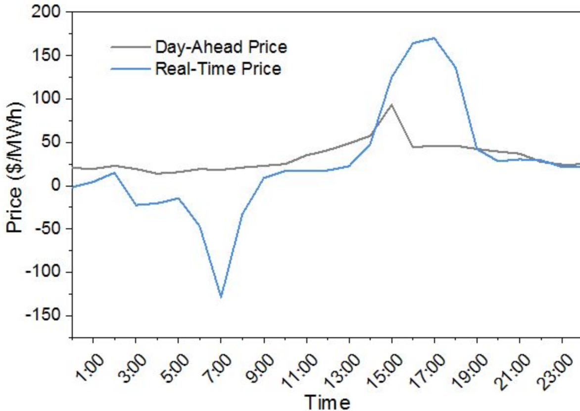
Figure 10: LMP for Maine Node 06/11/2017 55
