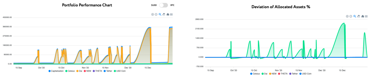
Figure 8: Rebalancing Backtest
