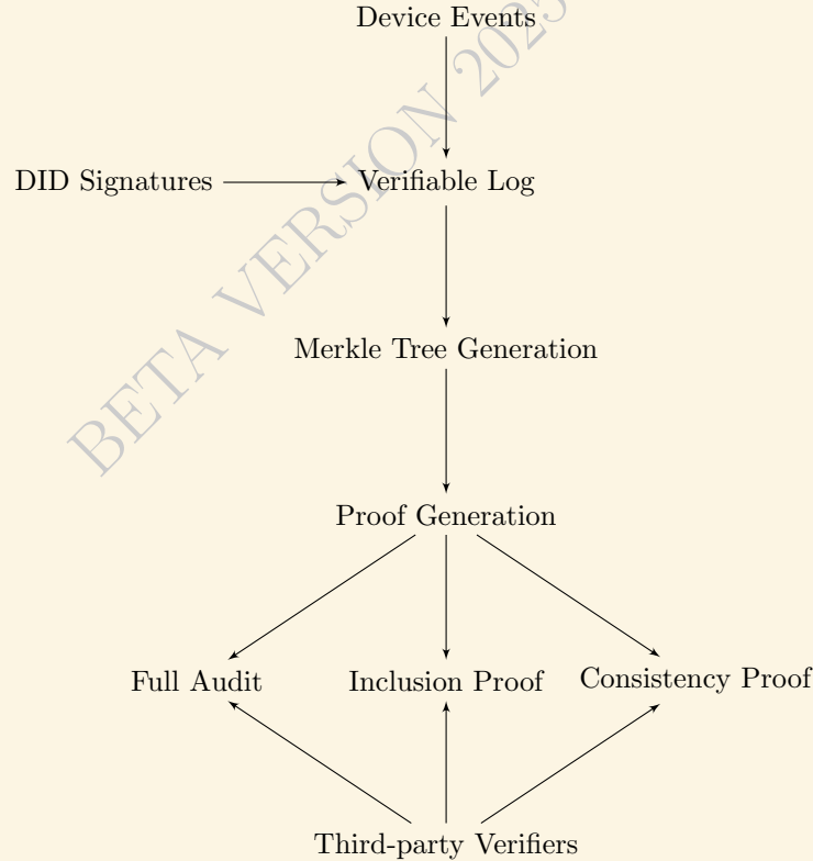
Figure 2: Verifiable Log System
