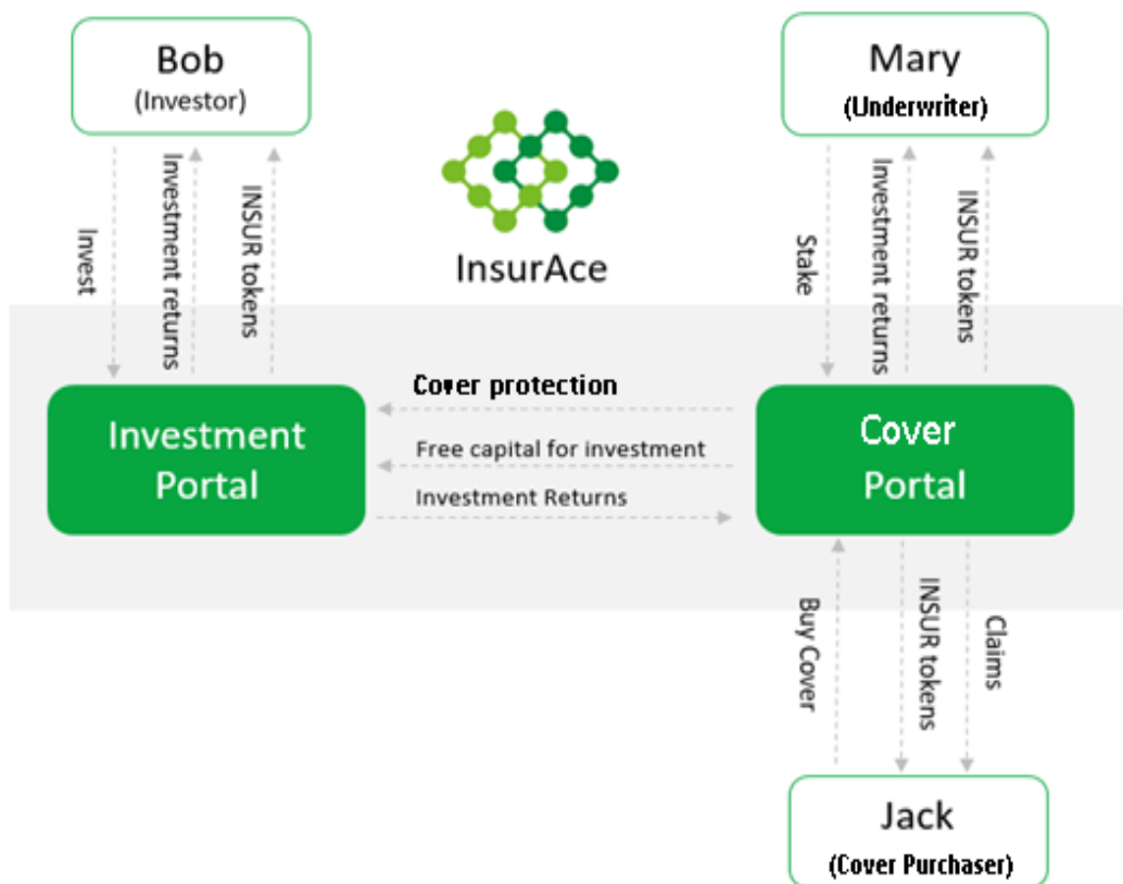
Figure 5 Use Cases
