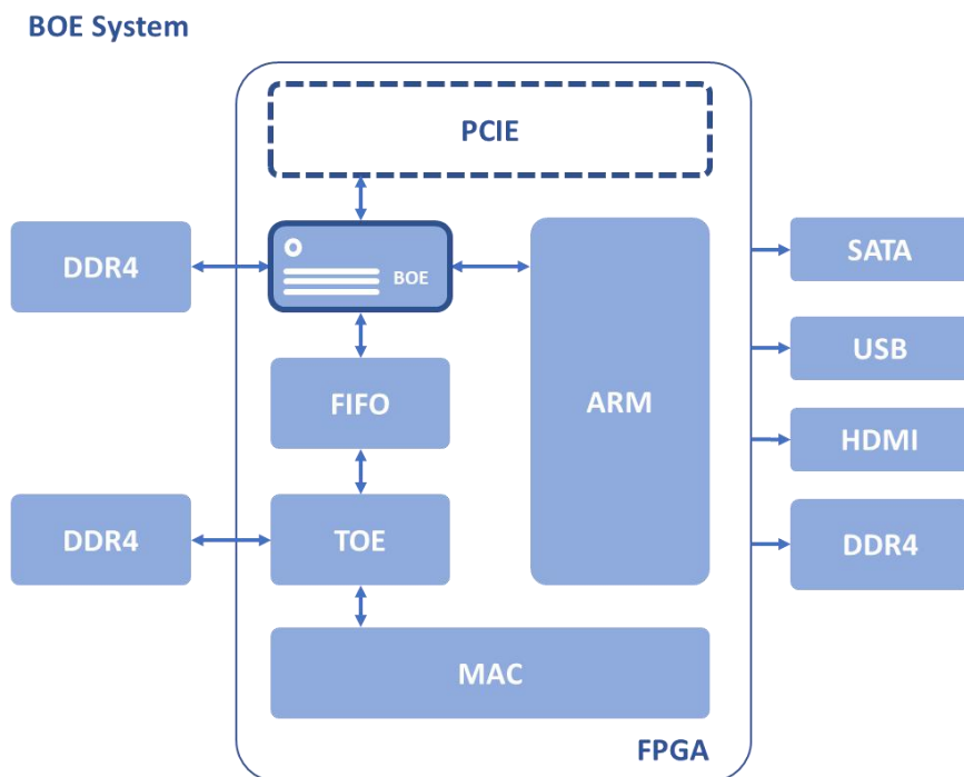
BOE Board Schematic
